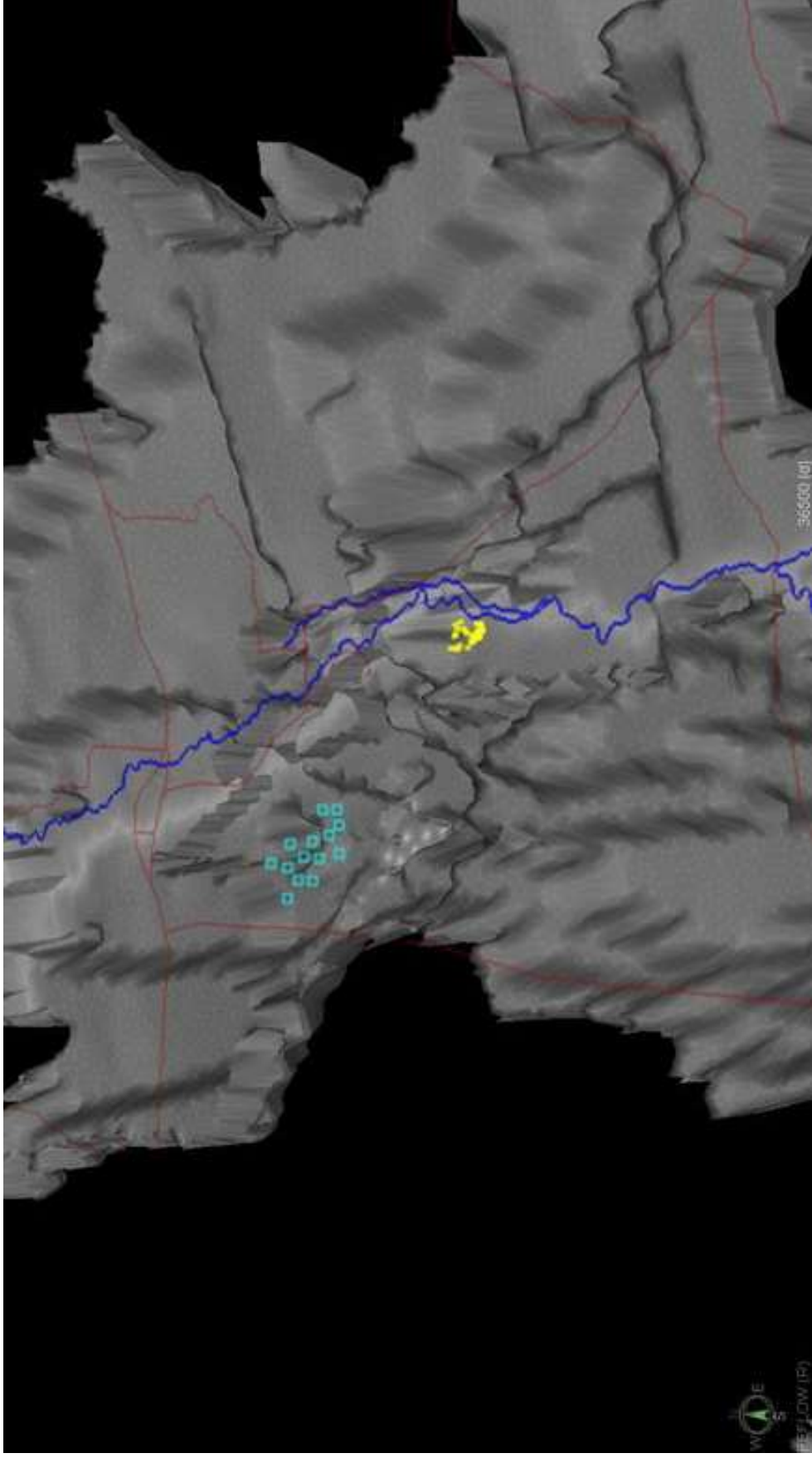
Figure 9. Modeled bedrock surface (from original Modflow model). The cyan symbols are Vigneto pumping wells, while yellow symbols are St. David Cienega spring. Roads are shown for reference (red). A notable trough exists, connecting the Benson and Huachuca basins (west of San Pedro). The Tombstone basin is shown east of the San Pedro river.
